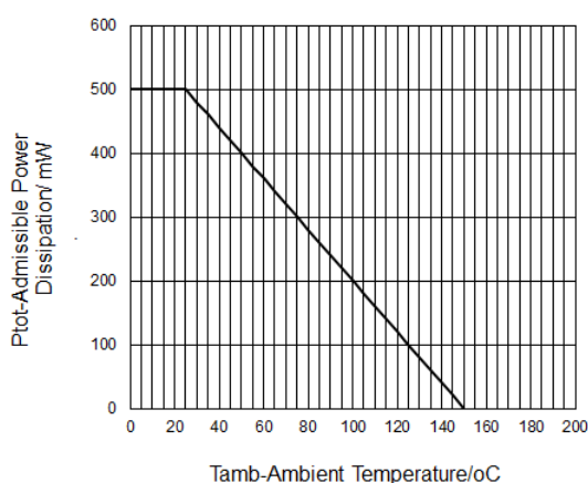
Figure 2. Power De-rating
